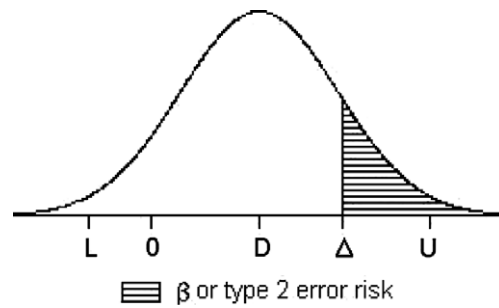
Fig. 4. Illustration of the type 2 error risk \beta in an RCT showing a difference D in effect, which is not significant, since zero (0) difference lies between the lower (L) and upper (U) 95% confidence limits. The type 2 error risk of having overlooked an effect of \Delta is substantial.
